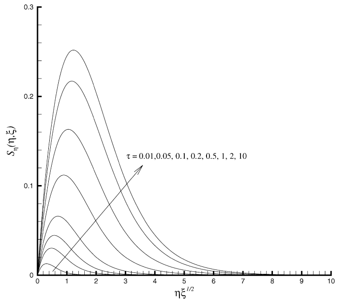
Fig. 10. The variation of the velocity profile S_\eta(\eta, \xi) for c = 0.5 and Pr = 0.72 when h = -1.5 .
